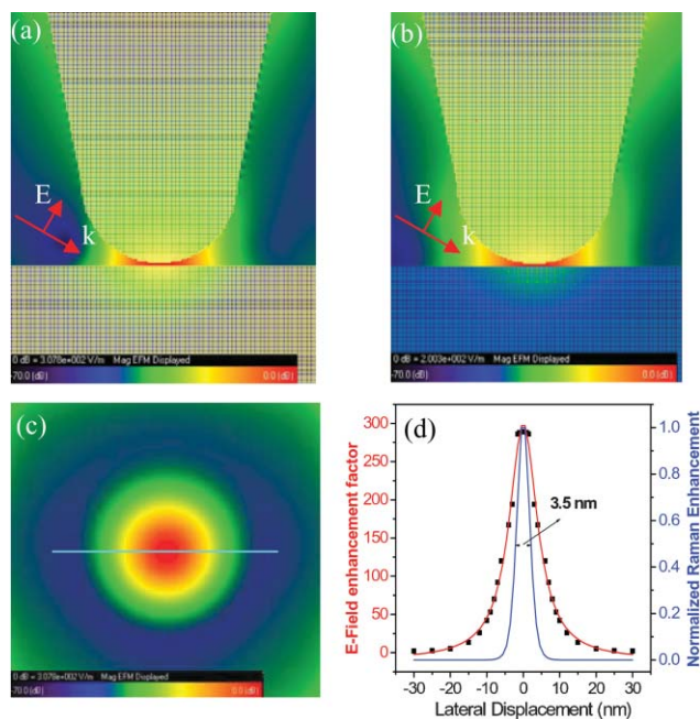
Fig. 19 FDTD calculation of the field distribution for the combination of Au tip and Au (a, c, d) and Pt (b) substrates: (a) Au tip and Au substrate; (b) Au tip and Pt substrate; (c) field distribution in the plane 0.5 nm above the substrate; (d) the line profile of the electric field enhancement and normalized Raman enhancement for the line indicated in (c). The incident direction and polarization of the laser is indicated in the figure. The tip radius is 20 nm placed 1 nm above the substrate.
