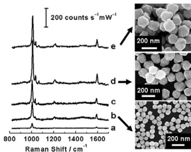
Fig. 12 SER spectra of pyridine adsorbed on Au@0.7 nm Pd/GC with different Au core sizes in 0.01 M pyridine and 0.1 M NaClO 4 solution: (a) 40 nm, (b) 80 nm, (c) 120 nm, (d) 135 nm, (e) 160 nm. Shown on the right side are the typical SEM images of nanoparticles with a diameter of 80 nm, 135 nm and 160 nm.
